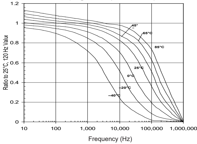
ESR vs. Temperature and Frequency 220 µF @ 50 Vdc (10 X 10.2 mm)
